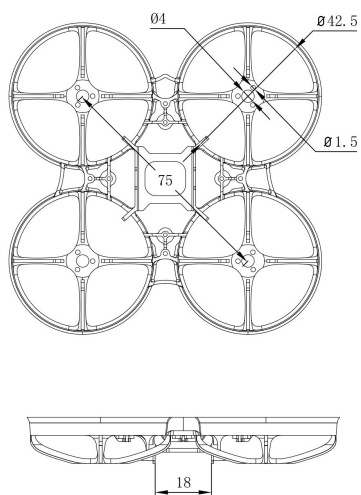
Petrel 75Whoop V2 Size diagram
