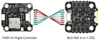
F405 V4 Flight Controller
